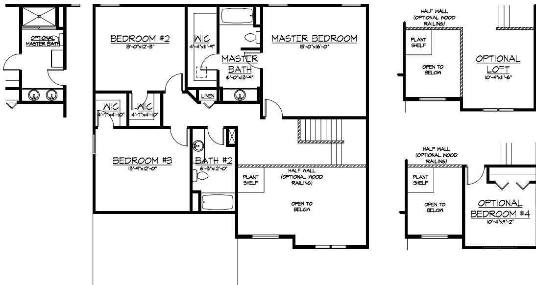
2ND FLOOR PLAN 1036 SQ. FT. (LOFT & BEDROOM #4 OPTIONS ADD 132 SQ. FT. EACH)
