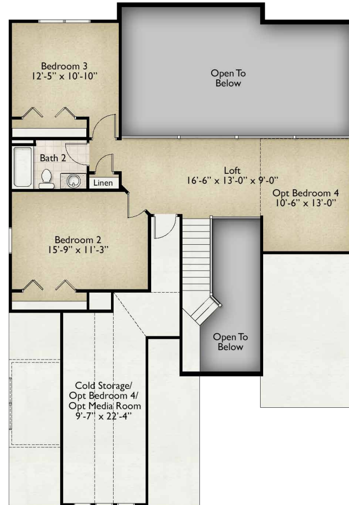
2nd Floor
