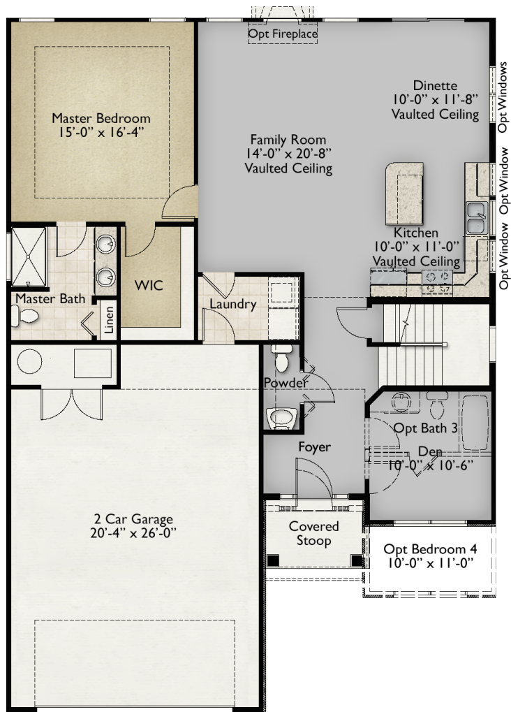
1st Floor
